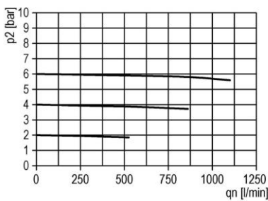
flow characteristic
